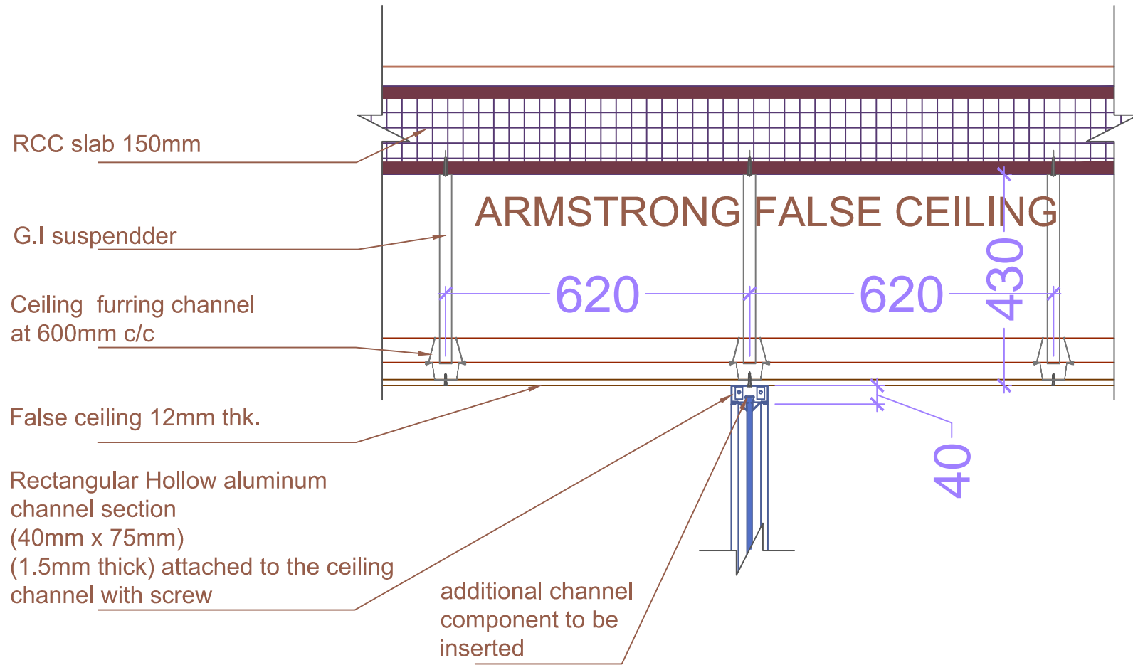
ARMSTRONG FALSE CEILING TYPICAL SECTION
