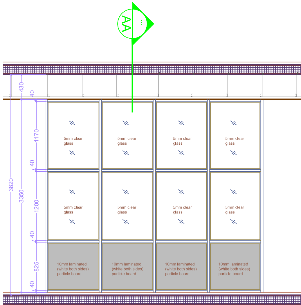
SECTIONAL ELEVATION
